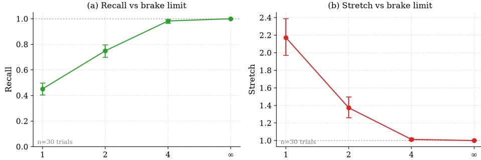
Figure 5: Single-broker brake sweep: recall and stretch against brake limit, 95% bootstrap CIs over 30 trials (data in Table 2).
