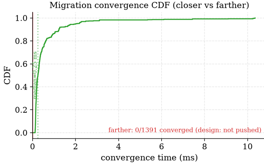
Figure 8: Cumulative distribution of convergence time for closer-class migrations. Farther-class migrations do not converge and are absent from the distribution.
